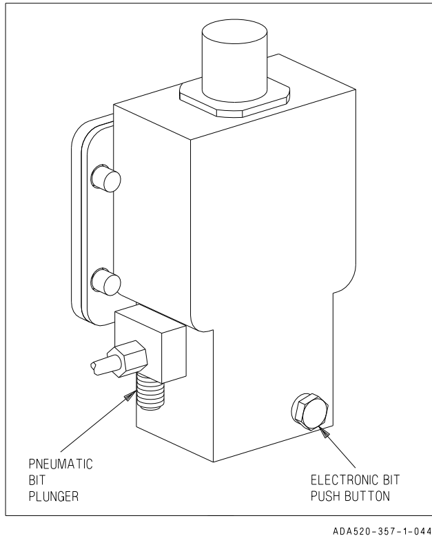
Figure 2-33A. OBOGS Monitor
