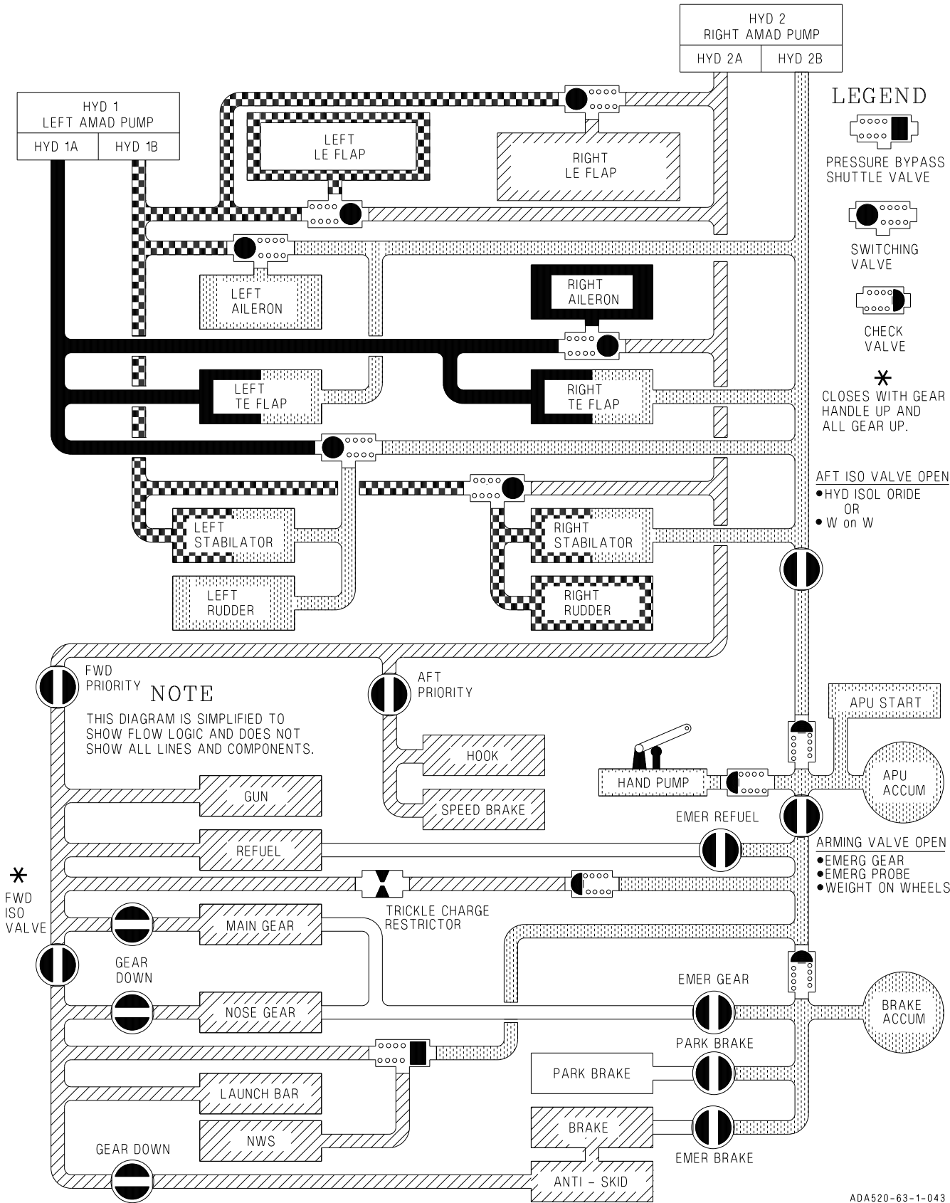
Figure 2-9A. Hydraulic System
