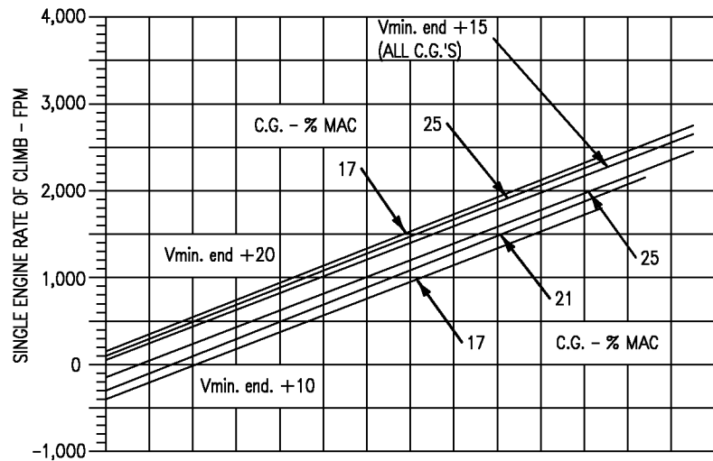
Figure 11-33. Single Engine Rate of Climb - Takeoff Configuration - F404-GE-400 (Sheet 6 of 10)
