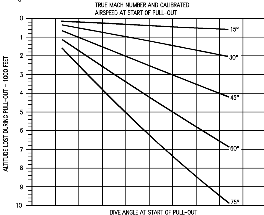
Figure 11-164. Dive Recovery - F404-GE-400 (Sheet 3 of 8)
