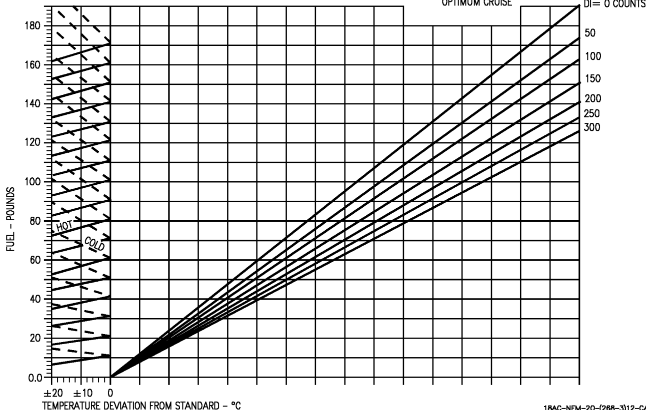
Figure 11-158. Normal Descent - One Engine Operating - F404-GE-400 (Sheet 3 of 4)
