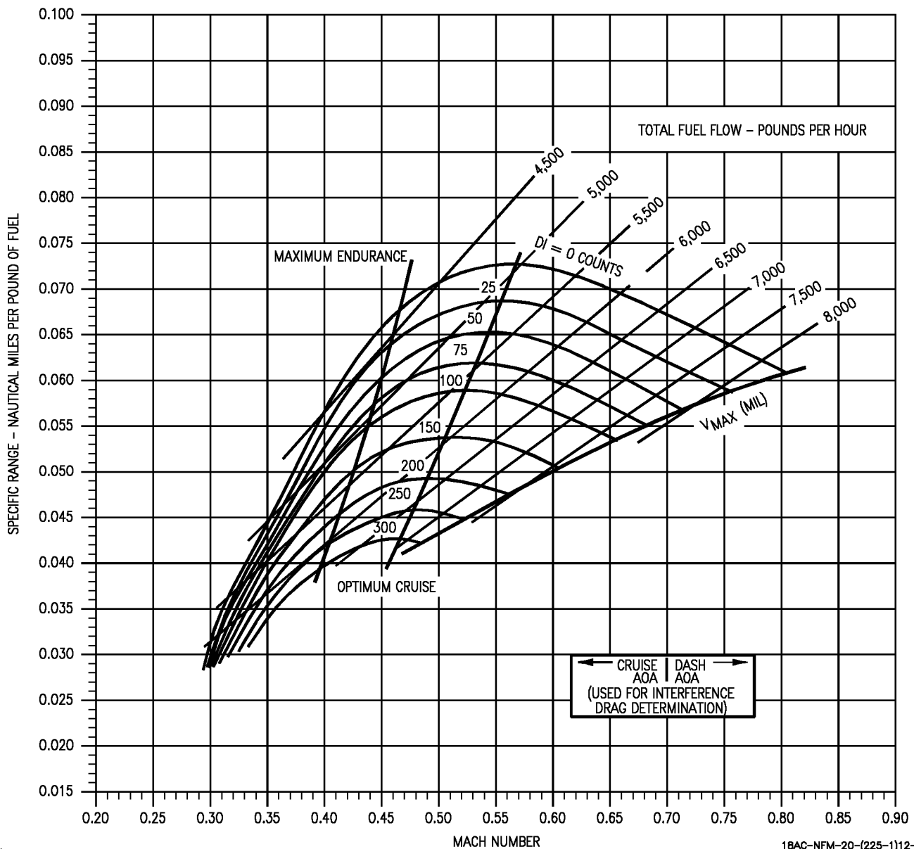
Figure 11-120. Specific Range - One Engine Operating - 10,000 Feet - 42,000 Pounds - F404-GE-400
