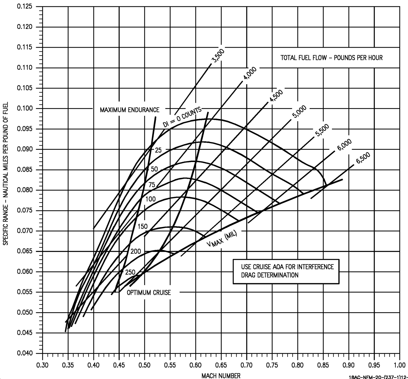
Figure 11-132. Specific Range - One Engine Operating - 20,000 Feet - 34,000 Pounds - F404-GE-400
